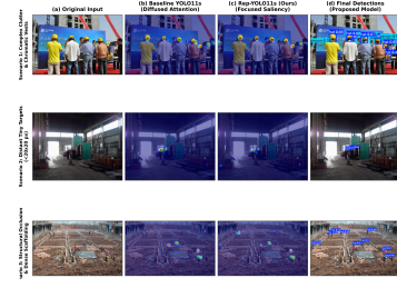
Fig. 4. Empirical Grad-CAM saliency maps across challenging conditions: Row 1 (Complex Clutter & Vests), Row 2 (Distant Targets < 20 × 20 px), Row 3 (Structural Occlusion). (a) Input, (b) Baseline YOLO11s, (c) Rep-YOLO11s, (d) Detections.
